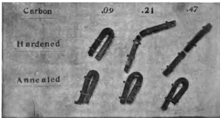
Fig. 67. The Hardening Power Increases with the Carbon-content.
